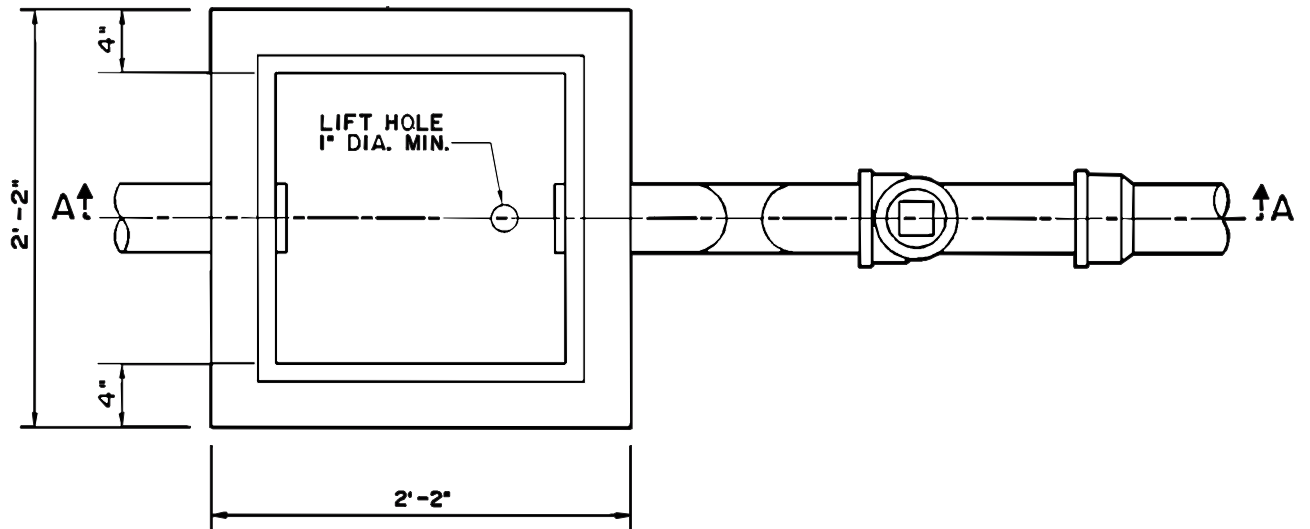
PLAN WITH COVER REMOVED
